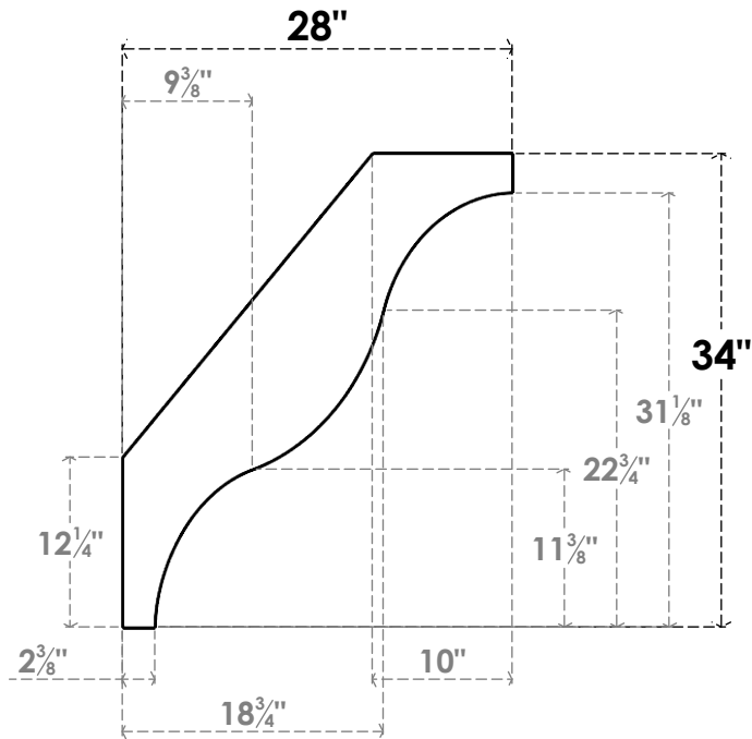
SIDE PROFILE
